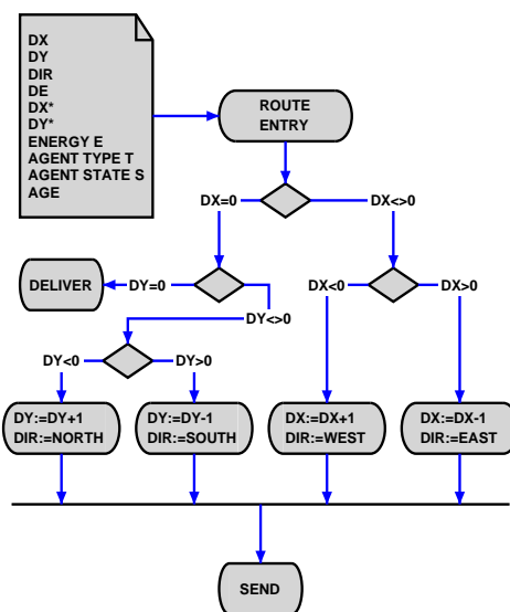
Fig. 2. UML activity diagram of the simplified message routing algorithm. Simple delta routing rules are applied to messages until the propagation vector is \Delta=(DX,DY)=(0,0) .
