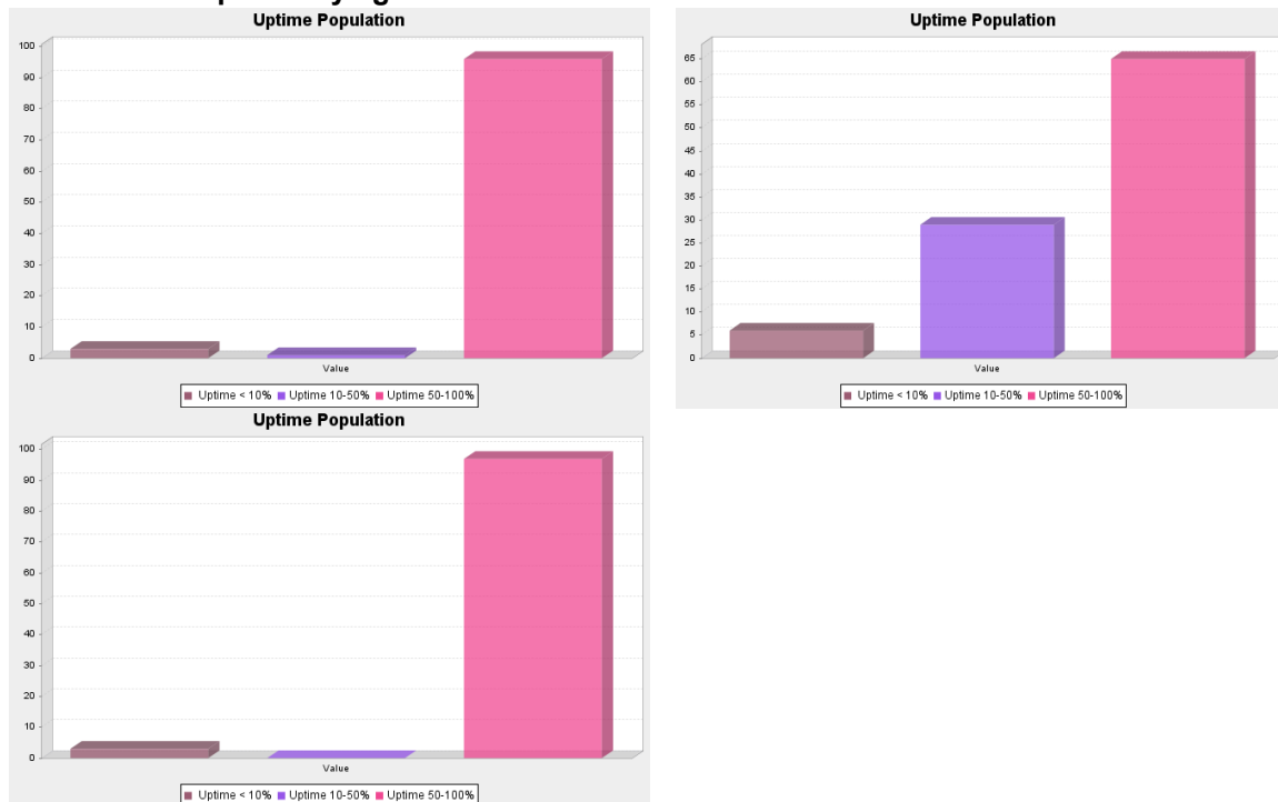
Fig. 9. Comparison of up-time distribution with (left) and without smart energy management (right). Each bar shows a up-time range relative to total running time, and the number of nodes (pay attention to different scales). The upper left chart shows the simulation using help-on-way and distribute agents, and for the lower left chart only help-on-way agents are used.
