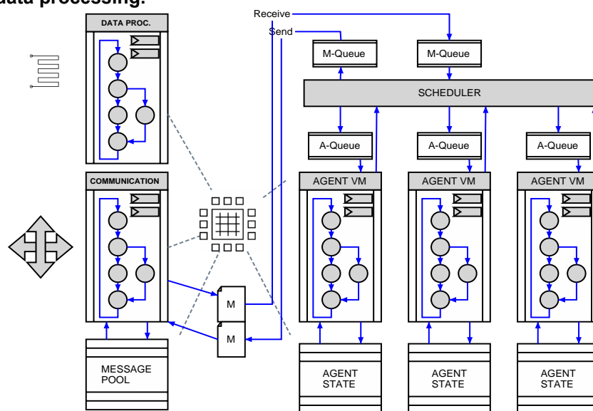
Fig. 3. Sensor node building blocks providing mobility and processing of multi-agent systems: parallel agent virtual machines, agent-processing scheduler, communication, and data processing.
