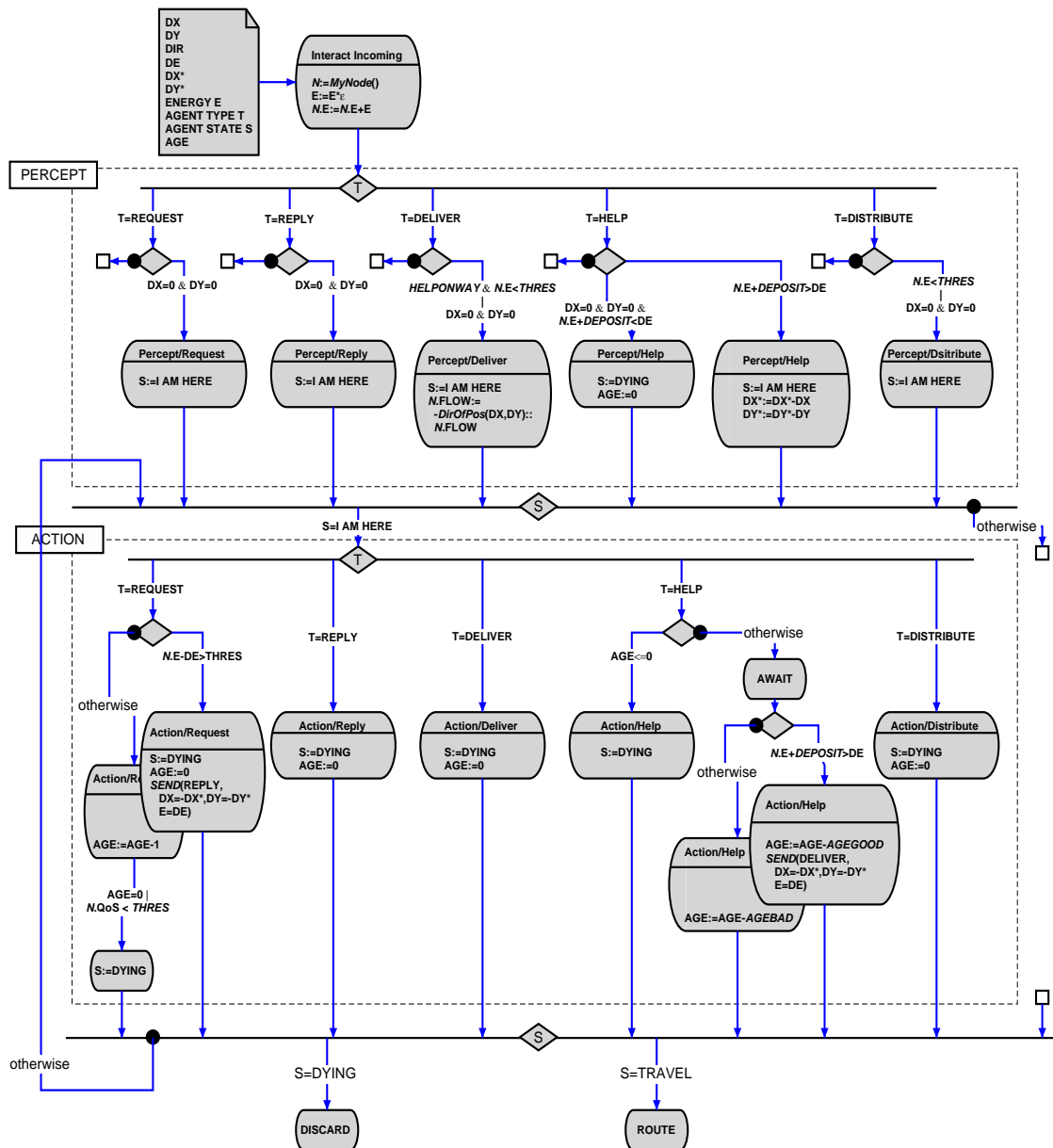
Fig. 4. UML activity diagram for the energy management agent. This super agent contains request, reply, help, deliver, and distribute agents implementing different behaviours.
