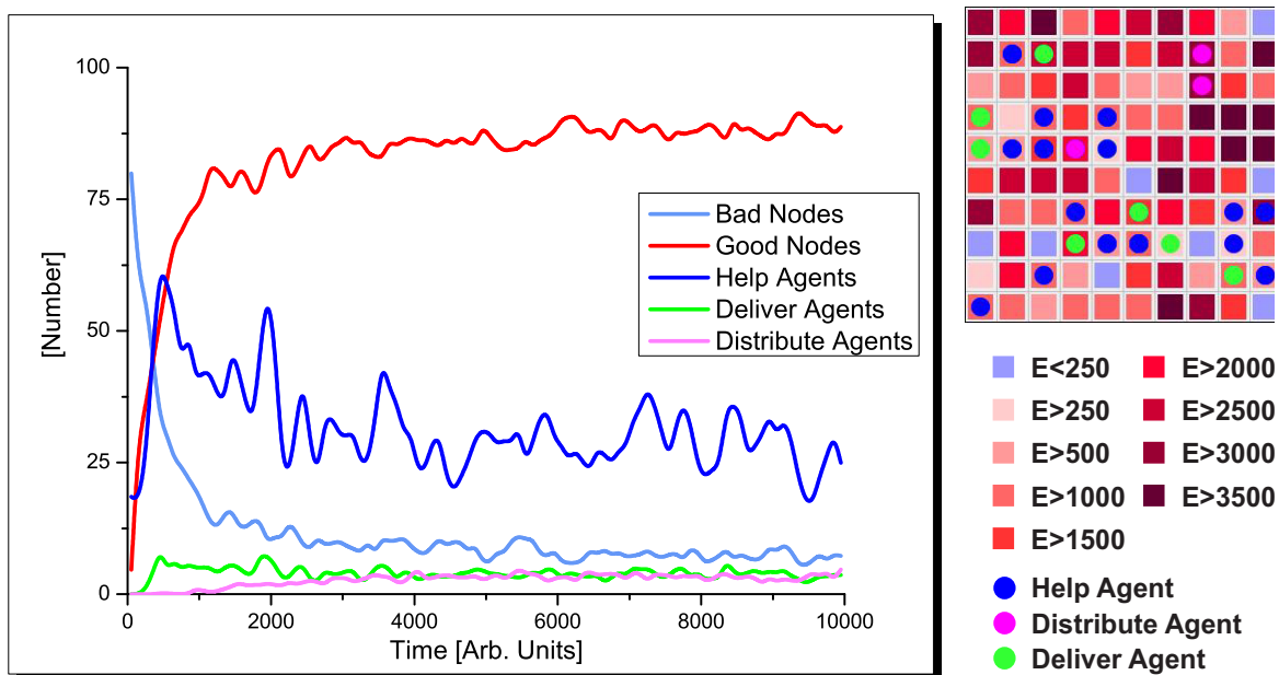
Fig. 6. Simulation results with energy management. Help, deliver, and distribute agents are used to compensate low-energy nodes. Shown are the spatial energy distribution after 10000 time units (right, with some agents) and the temporal population for bad and good nodes and agents (left).
