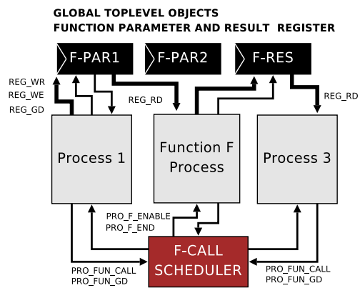
FIGURE 4: Shared function blocks are implemented with a process block and a function call scheduler. Only some of the interconnect signals are displayed.
