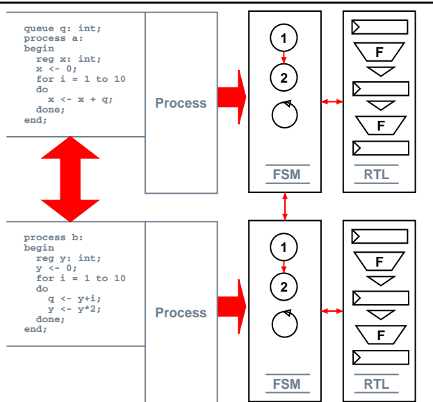
Figure 1. Mapping of the proposed multi-process model to FSM-RTL architecture using high-level synthesis.
