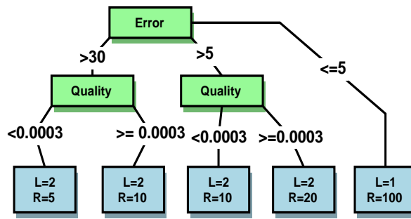
Figure 8. Decision tree used for energy optimization at runtime based on parameters. Input parameters: Error, Quality=Runtime/Error. Output parameters: Data processing rate R={1,5,10,20,100}, Algorithmic level L={P:1,PID:2}
