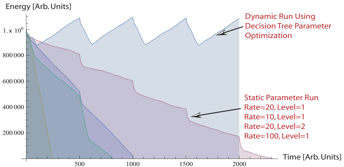
Figure 9. System simulation with different runtime behaviours using a decision tree which can be retrieved by machine learning methods. Parameters: Data processing rate={1,5,10,20,100}, Algorithmic level={P:1,PID:2}
