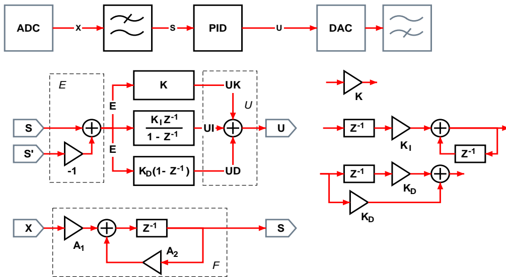
Figure 1. Composition and modelling of a digital control system with signal flow diagrams
